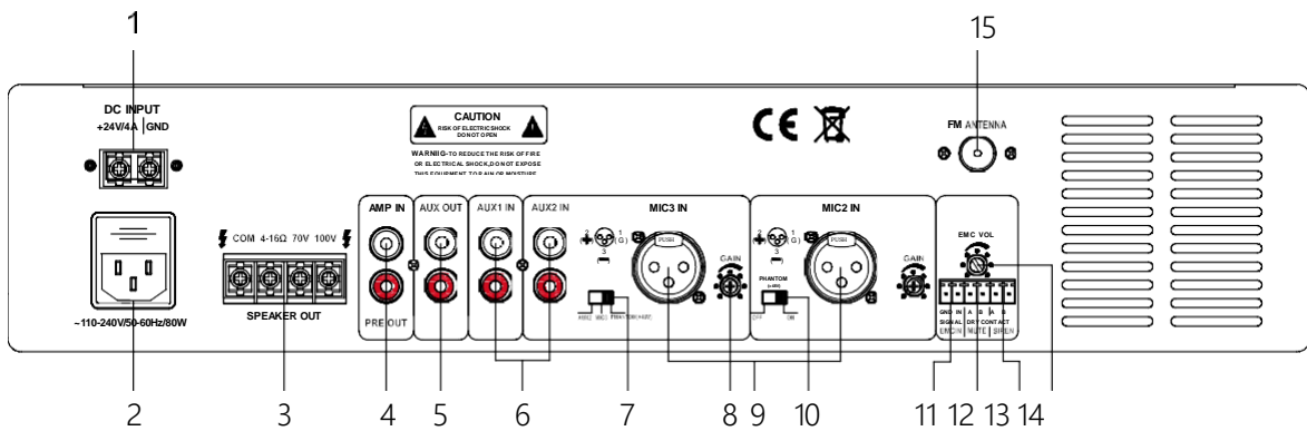
HIP-2060/HIP-2120/HIP-2250 Rear Panel
