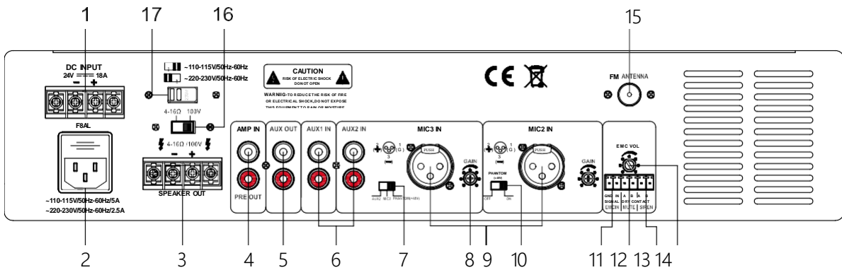
HIP-2350/HIP-2500/HIP-2650 Rear Panel
